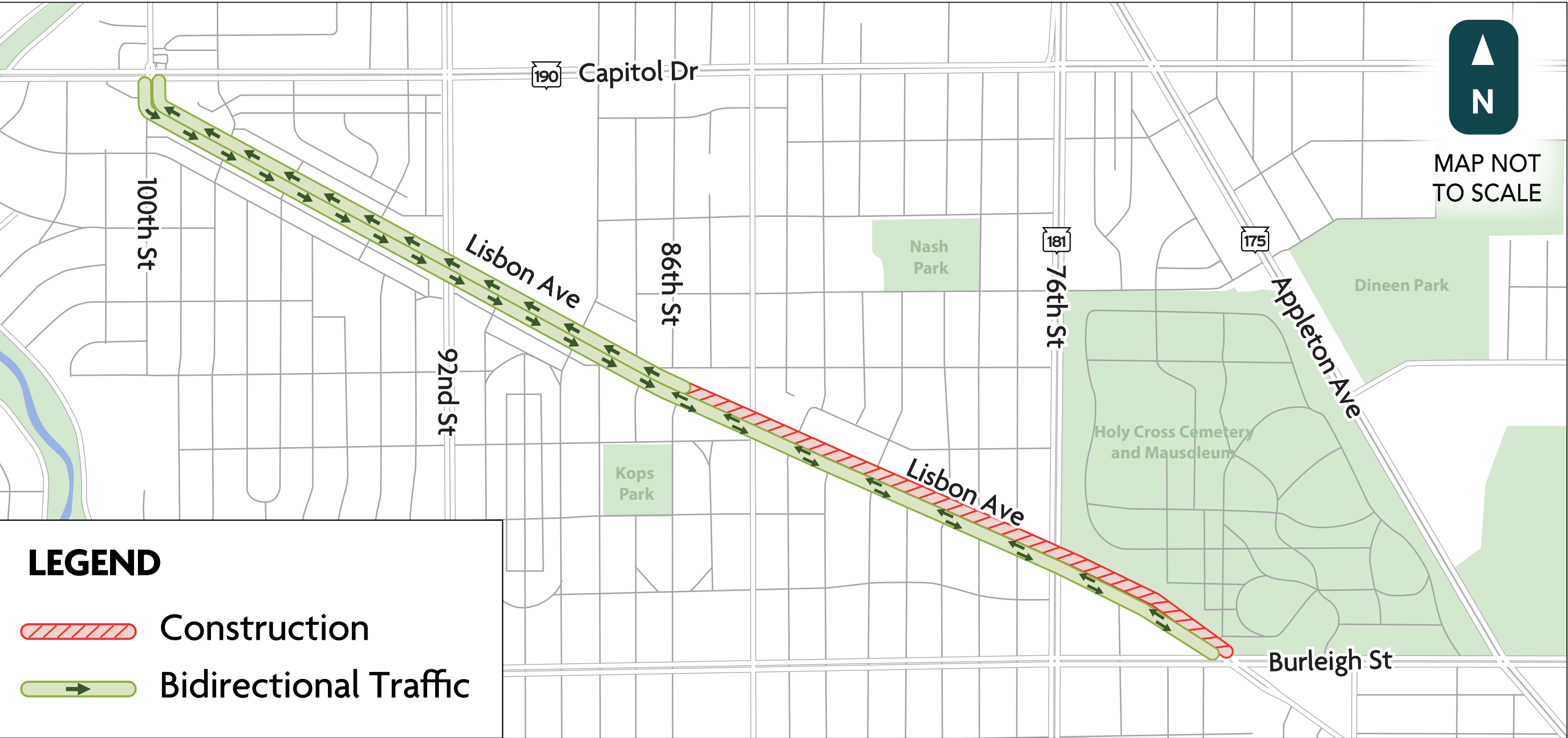
Detailed view of the traffic configuration during stage 3 of construction.
