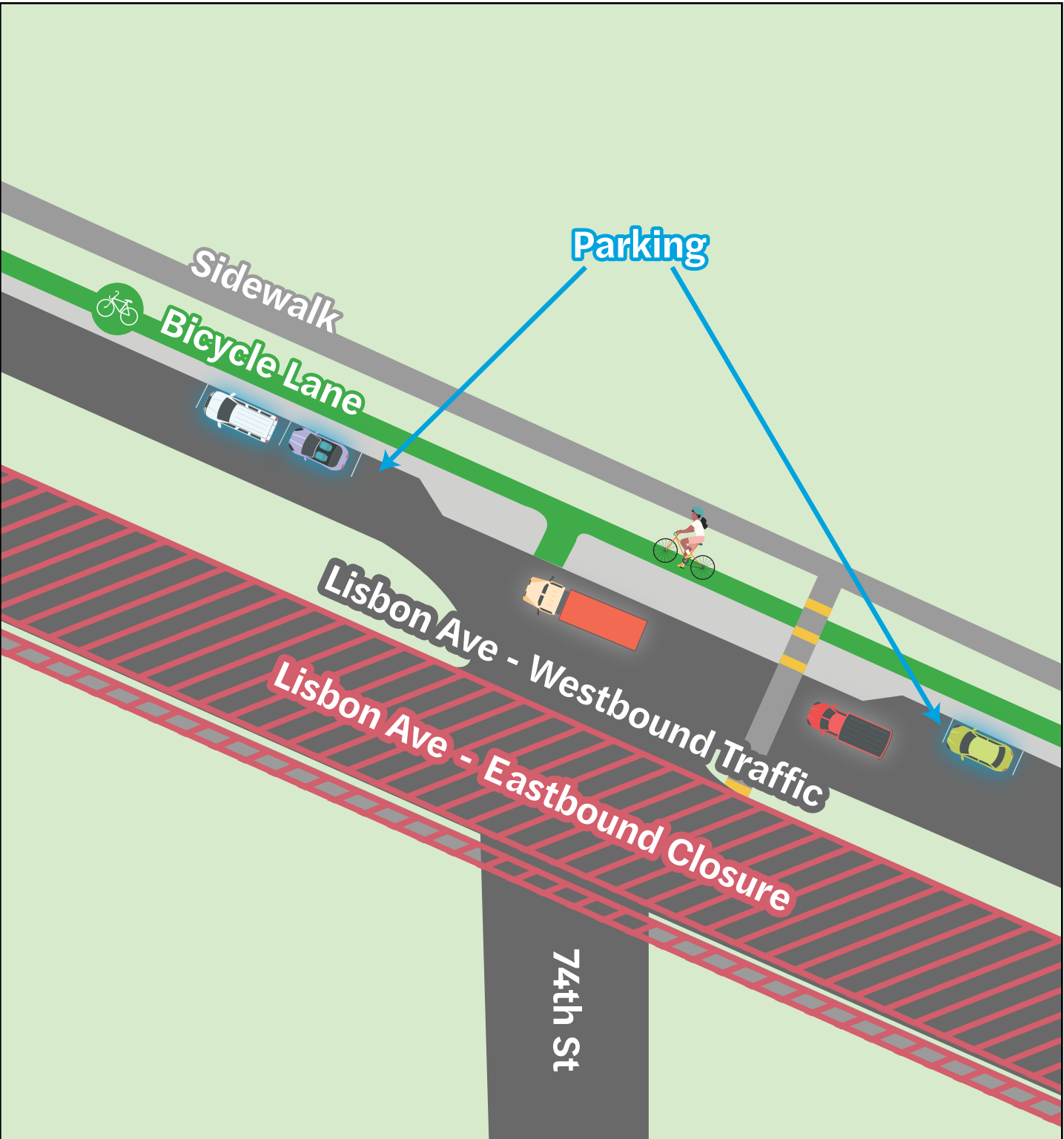
Detailed view of the traffic configuration during stage 4 of construction.
