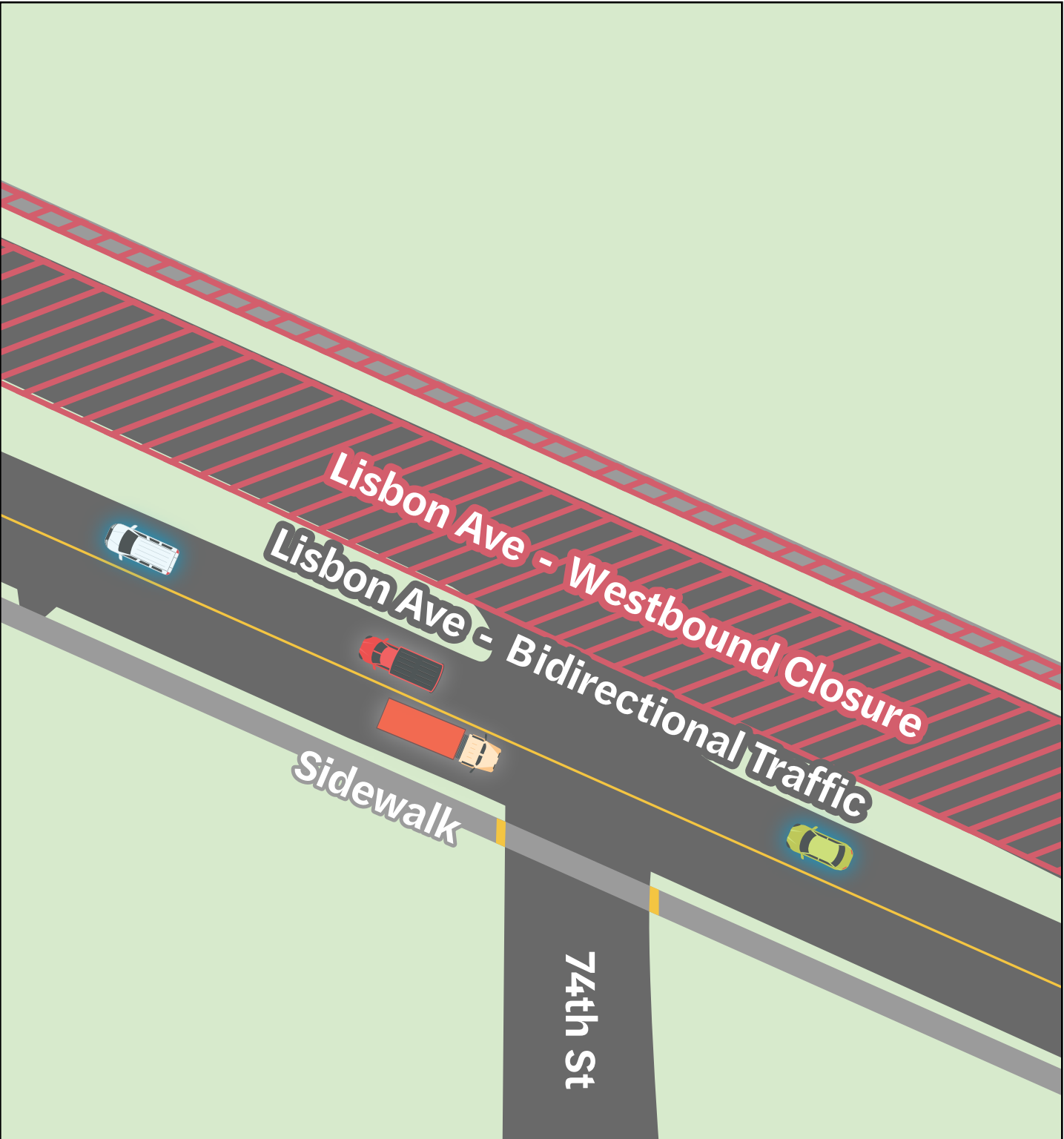
Detailed view of the traffic configuration during stage 3 of construction.
