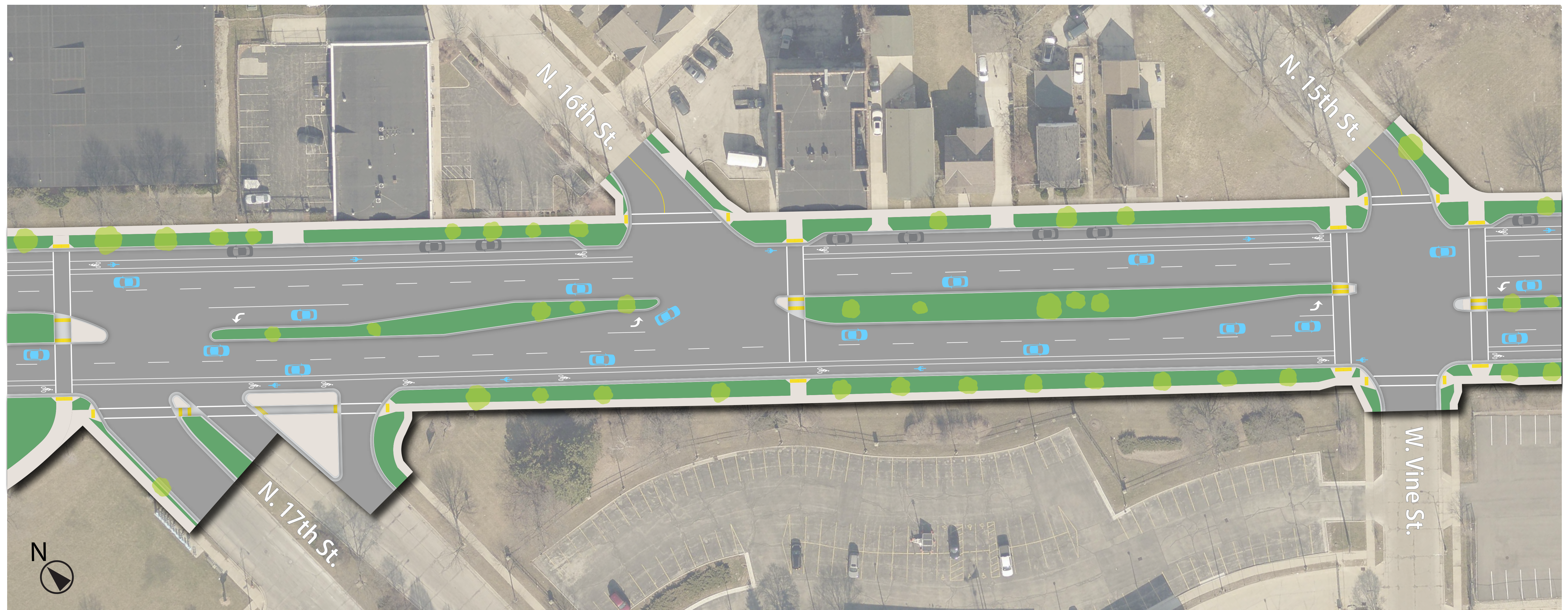
On Road Bike Lane Alternative - Facing West
