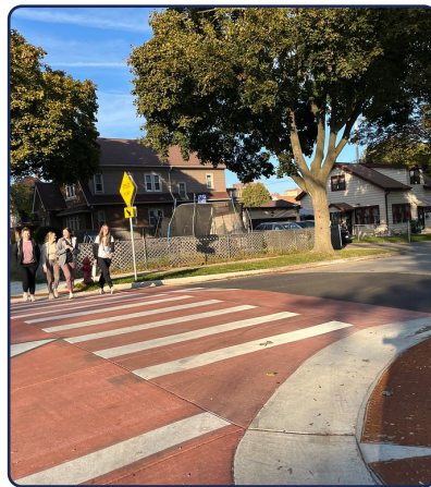
Raised crosswalk
