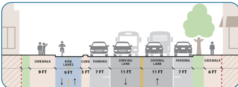
Example Cross Section (facing East on W. Center Street)
